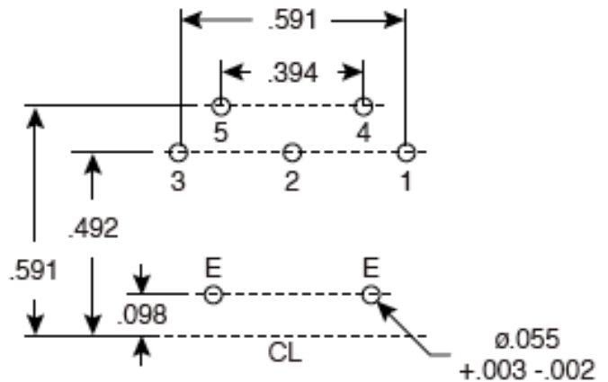
PCB Hole Layout Top View
